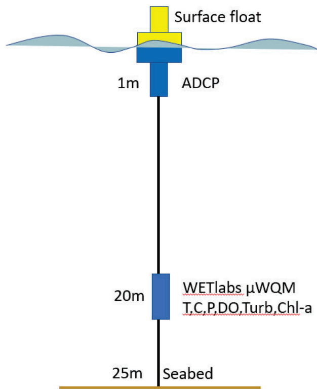
Figure 4.4: ADCP and WQM Configuration
