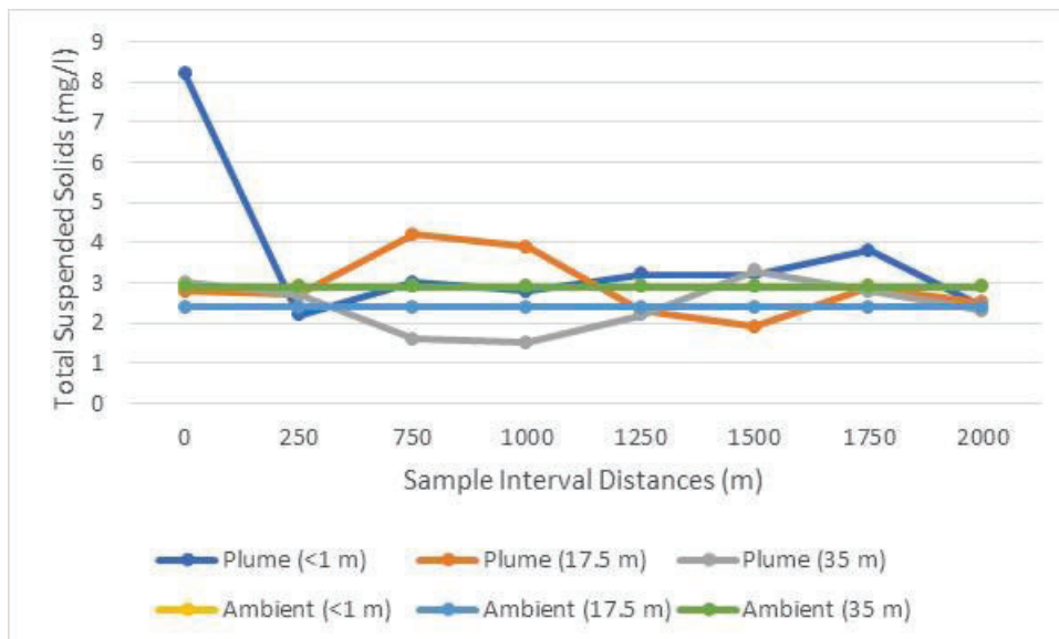
Figure 5.5: Transect One TSS (mg/l) Concentrations at 250 m Intervals from Plume Source Compared to Ambient
