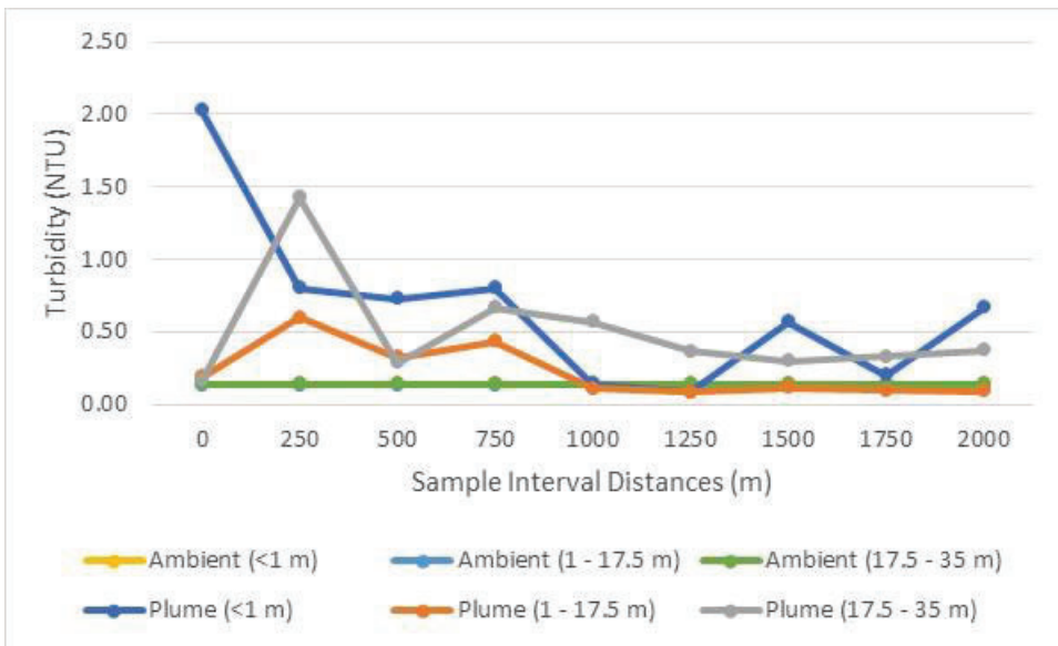
Figure 5.8: Transect Two Turbidity (NTU) Values at 250 m Intervals from Plume Source Compared to Ambient
