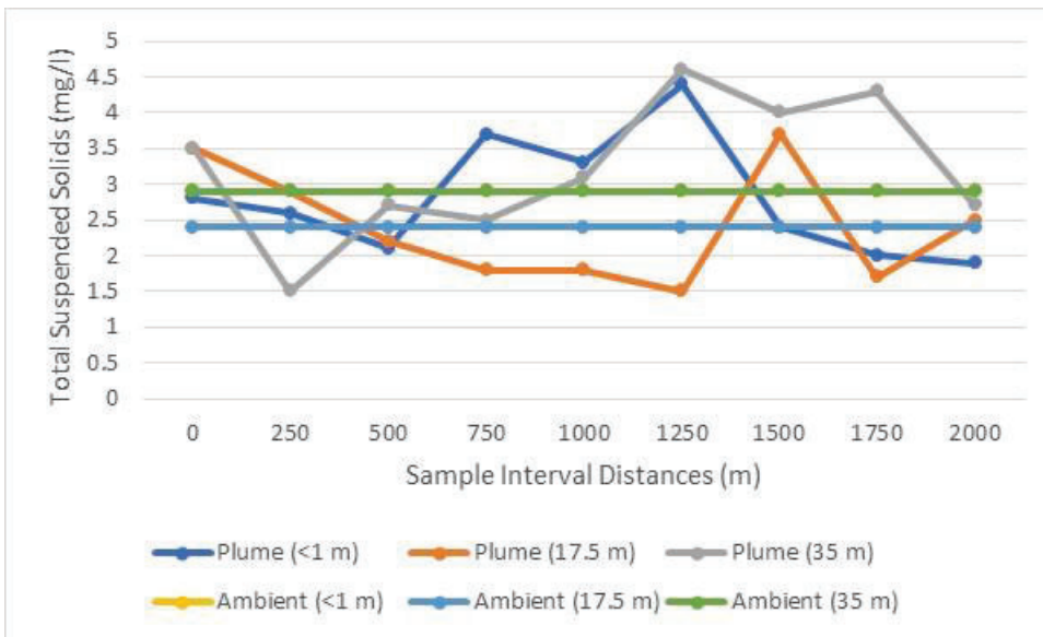
Figure 5.6: Transect Two TSS (mg/l) Concentrations at 250 m Intervals from Plume Source Compared to Ambient Note: The yellow line is not seen as it is beneath the blue ambient line
