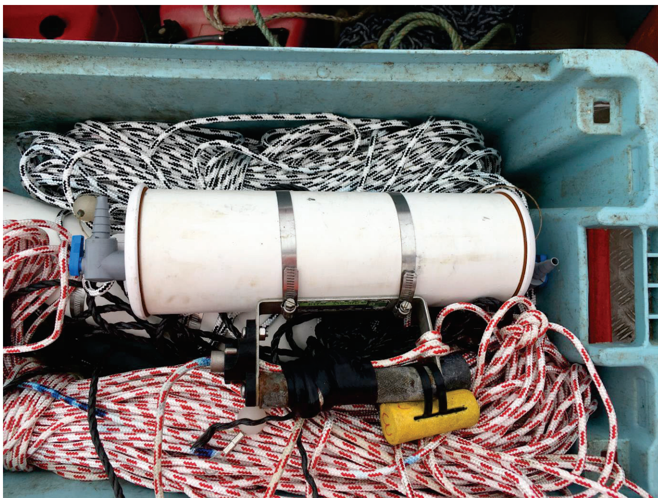
Figure 4.6: Van Dorn Grab used for Water Column Sampling
