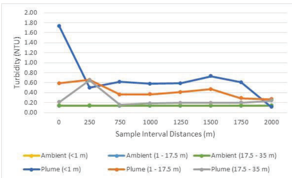
Figure 5.7: Transect One Turbidity (NTU) Values at 250 m Intervals from Plume Source Compared to Ambient
