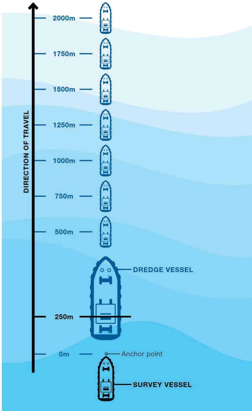
Figure 5.4: Overview of Sand Extraction Plume Survey Methodology and Intervals
